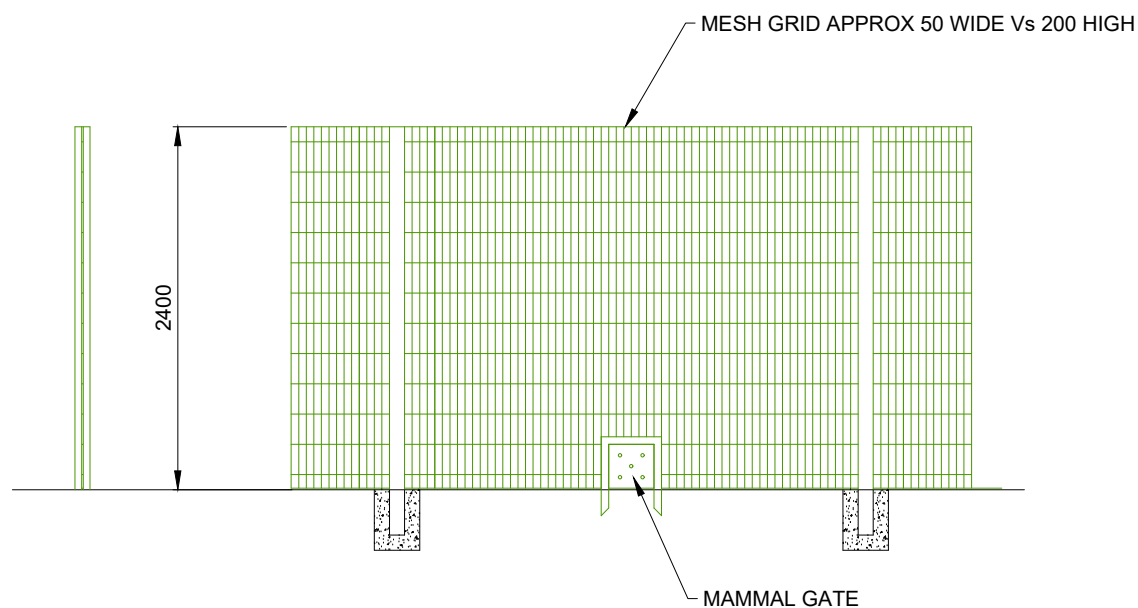
SECURITY FENCE END ELEVATION
