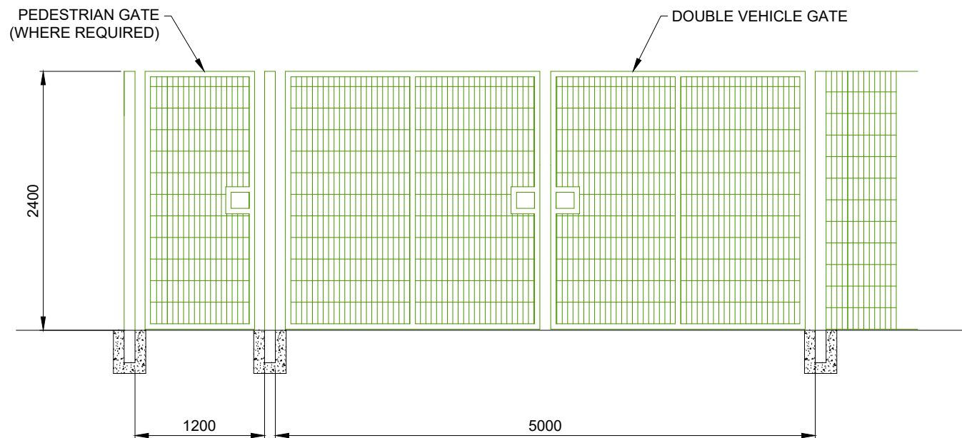
ACCESS GATE SIDE ELEVATION
