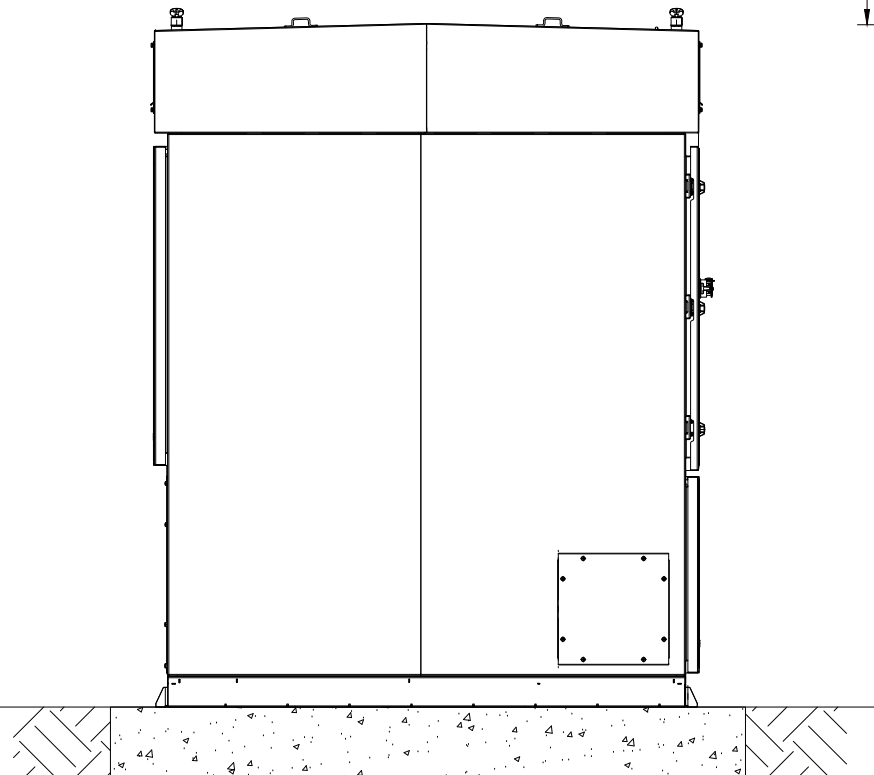
ELEVATION D
